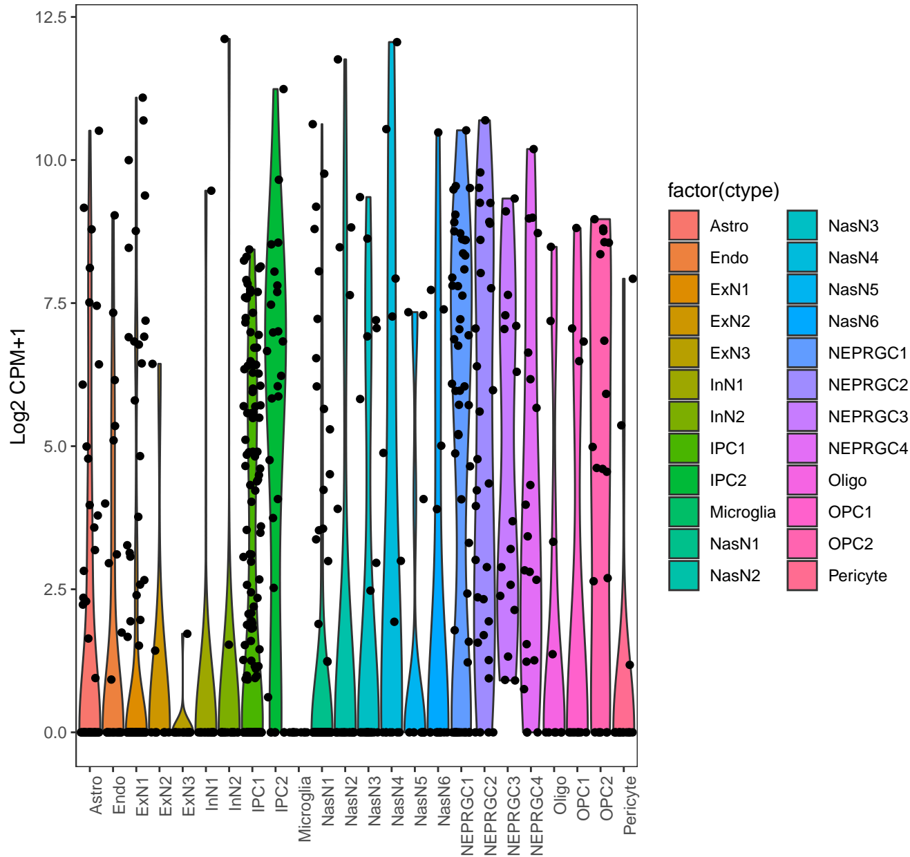
FIGN_ENSG00000182263 _Sestan_humanPrenatal
